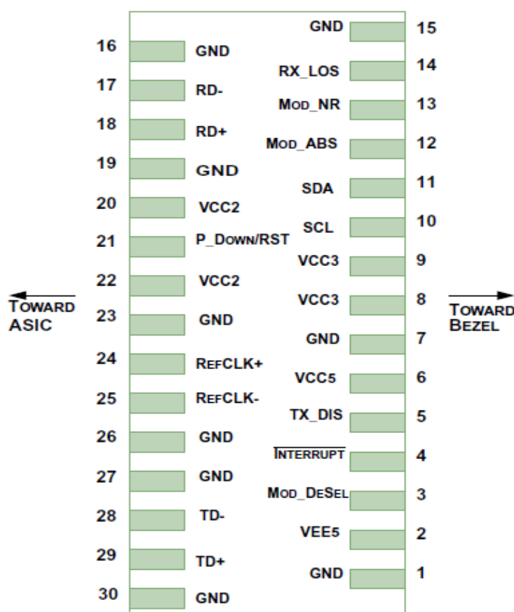
Diagram of Host Board Connector Block Pin Numbers and Name (Top View)
