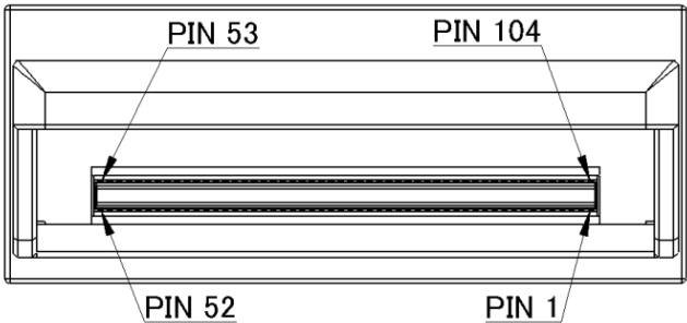
Figure 8. CFP2 Module Pad Layout
