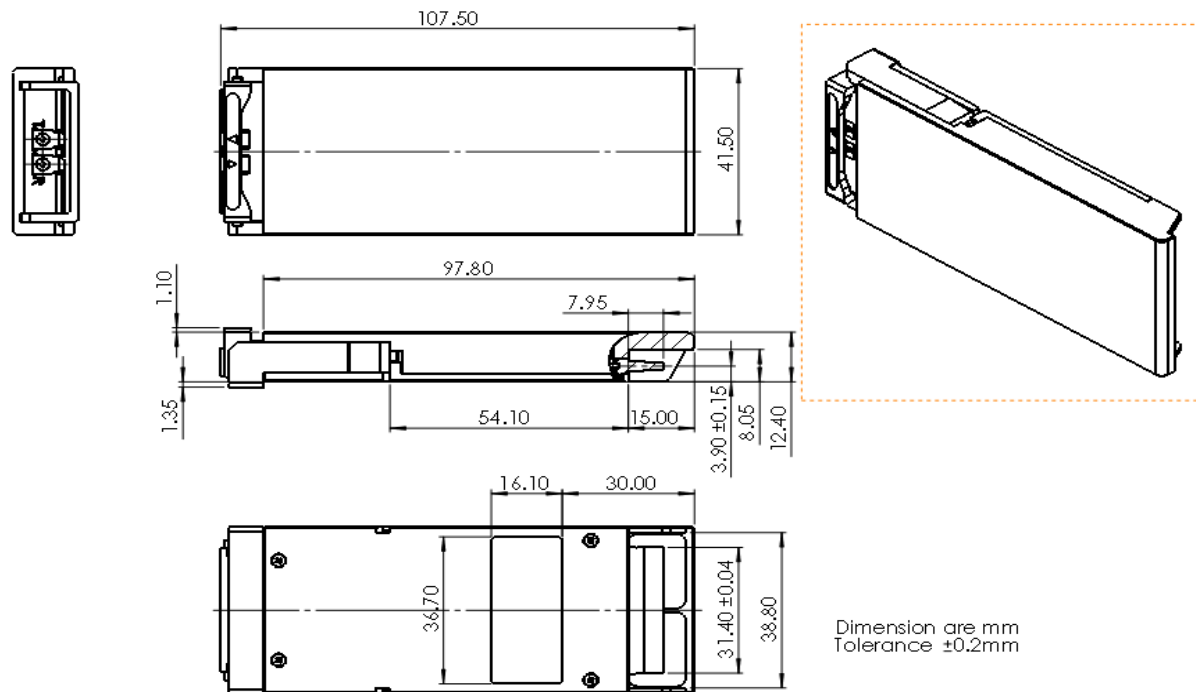
Figure 10. 100Gb/s CFP2 Mechanical Dimensions(unit:mm)
