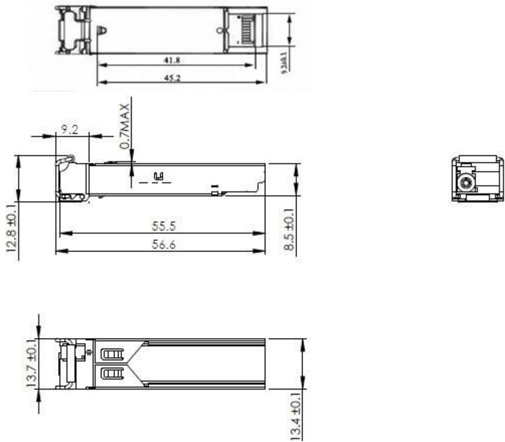
Mechanical Drawing
