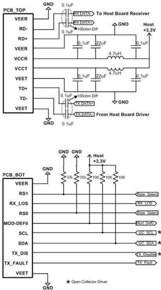
Recommended High-speed Interface Circuit
